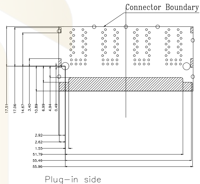
Keep-Out Area (Component Side View):
